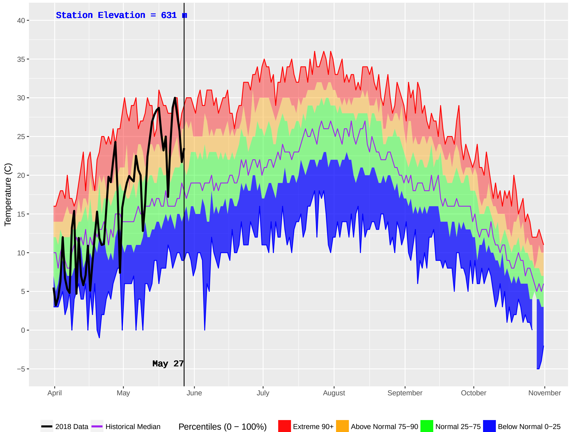
EAST BARRIERE (243) : Historical (1978–2016) and Current (2018) Noon Temperature
