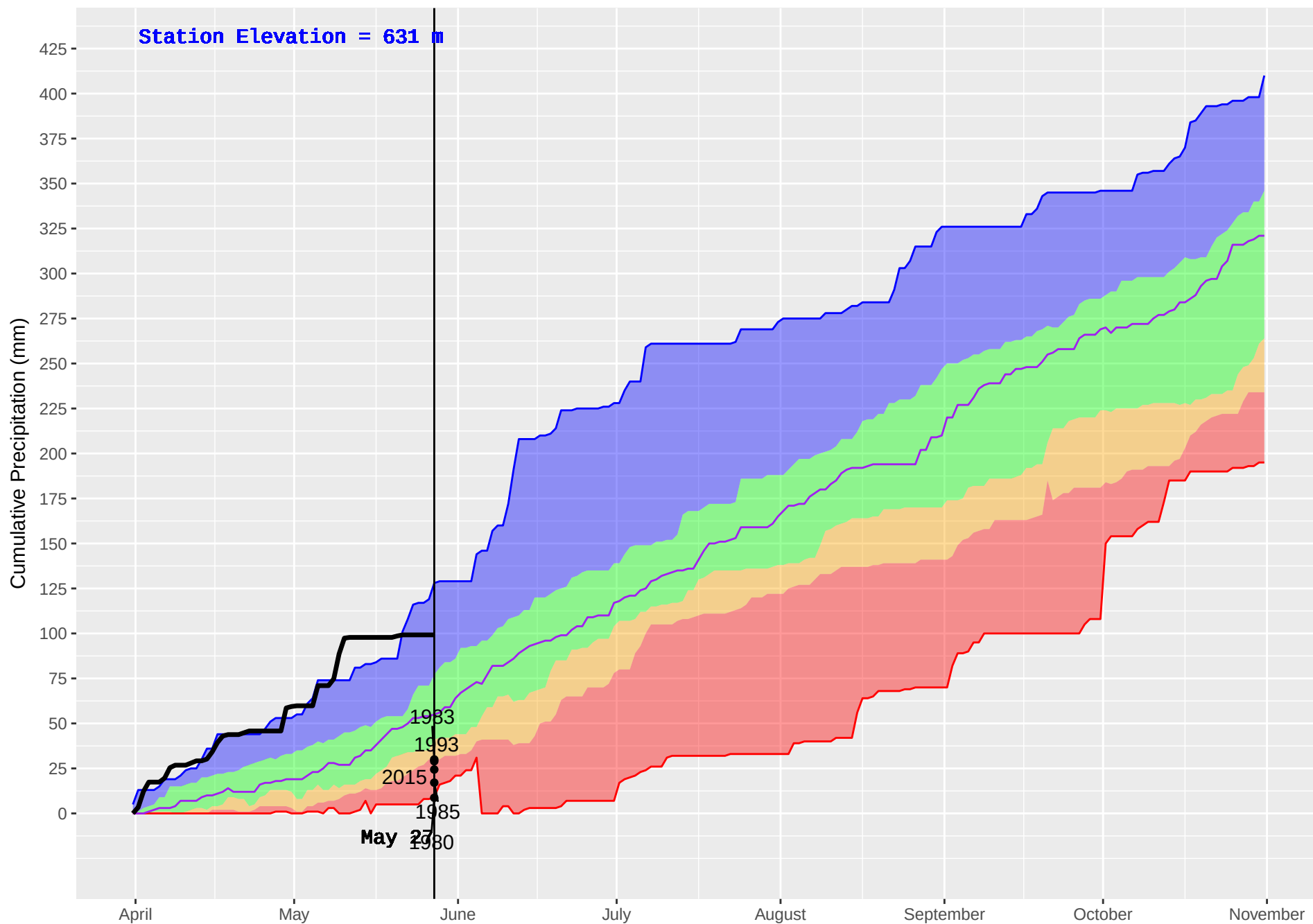
EAST BARRIERE (243) : Historical (1978–2016) and Current (2018) Noon Cumulative Precipitation
